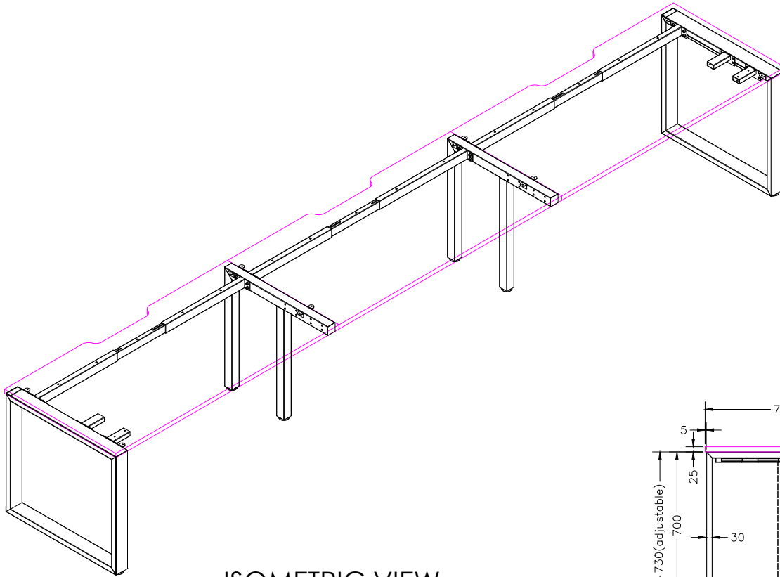
ISOMETRIC VIEW
