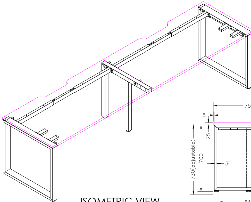
ISOMETRIC VIEW
