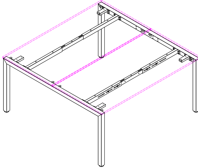
ISOMETRIC VIEW
