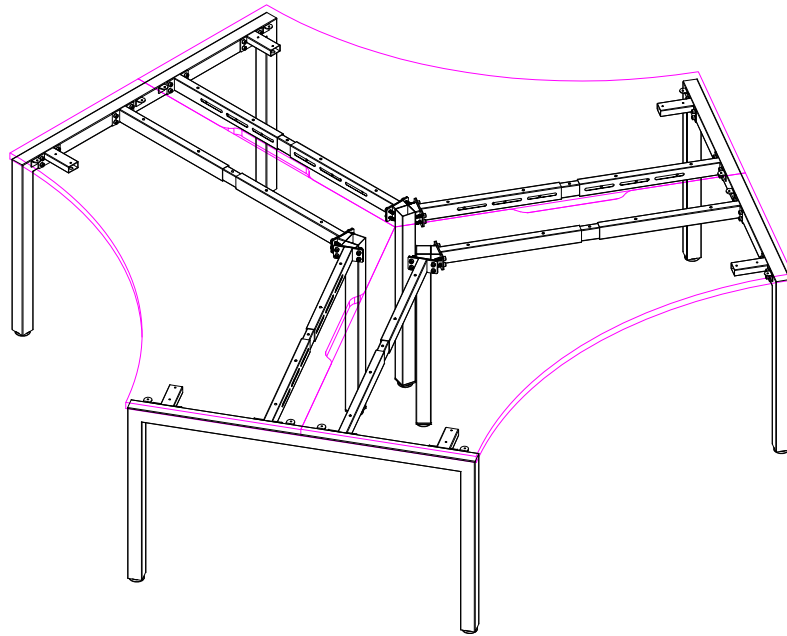
ISOMETRIC VIEW
