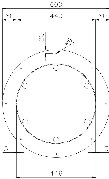
TOP VIEW
