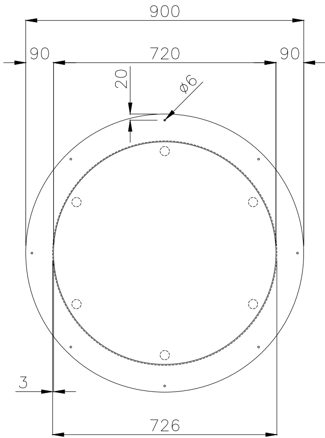
TOP VIEW
