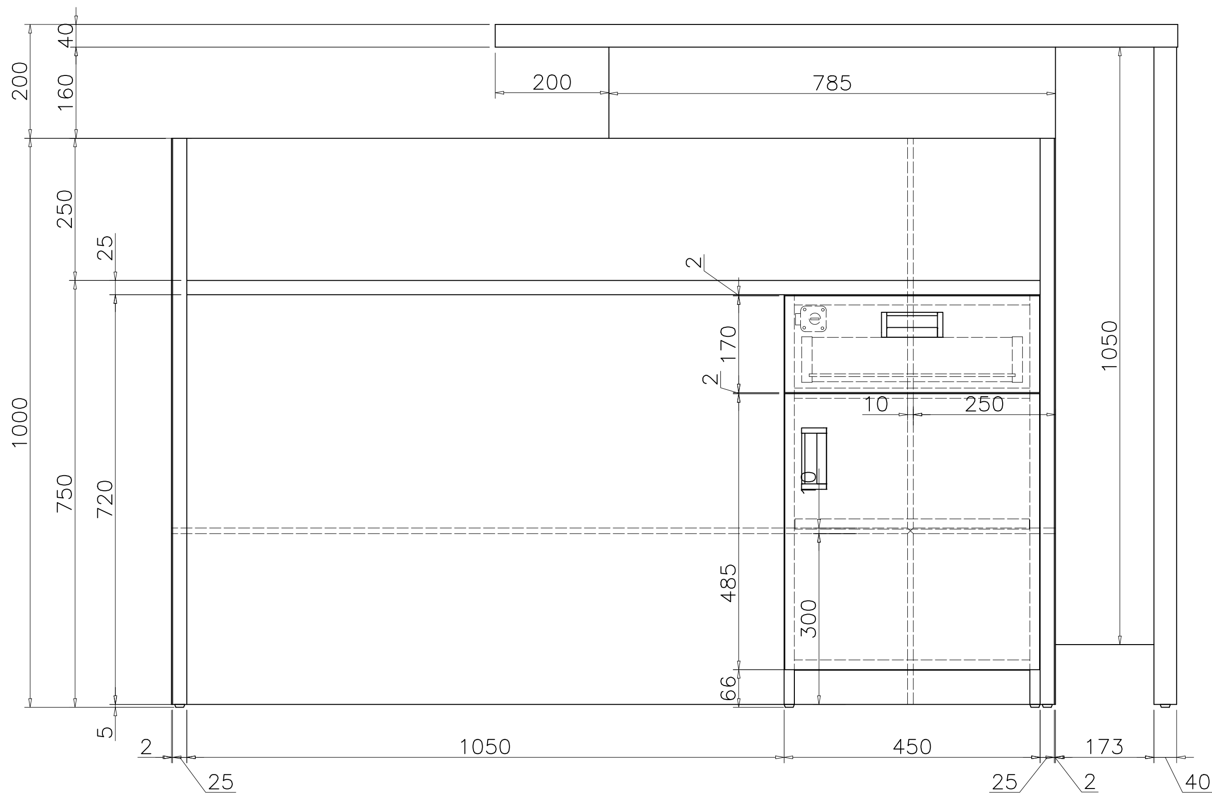
FRONT VIEW
