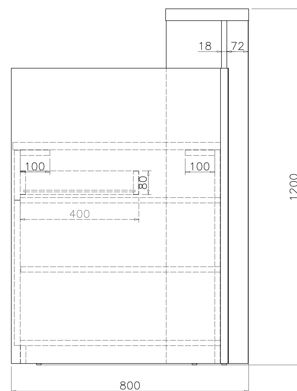
SIDE VIEW
