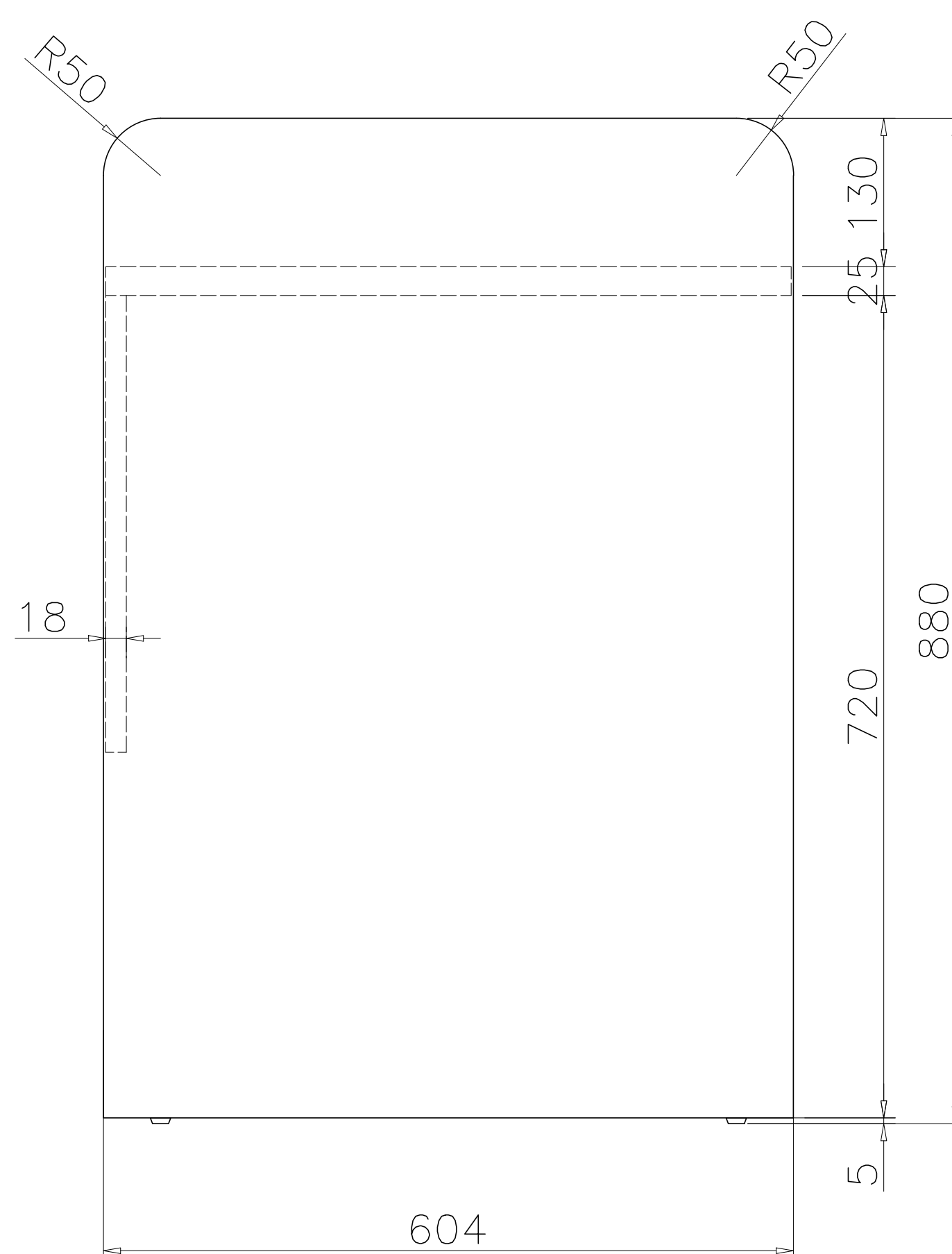
SIDE VIEW
