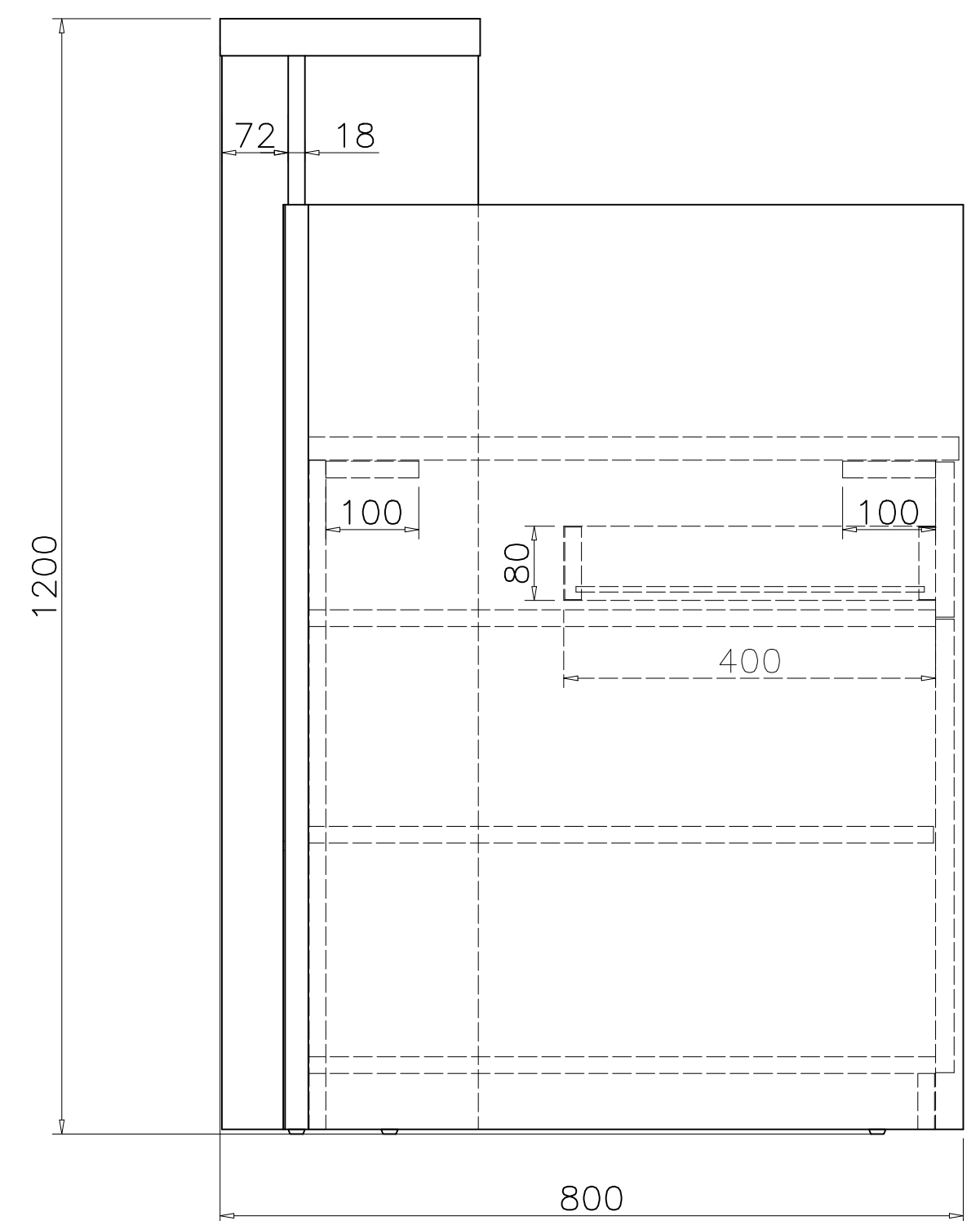
SIDE VIEW
