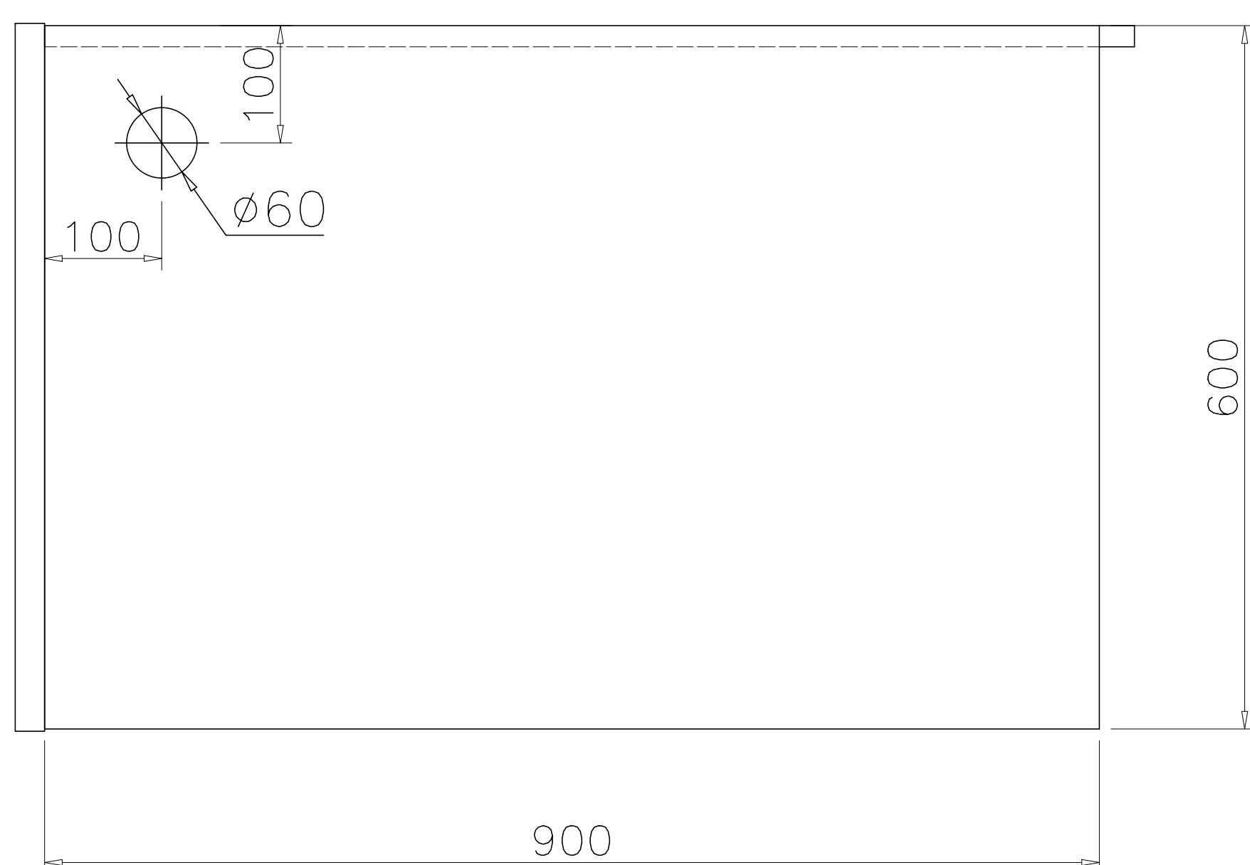
TOP VIEW
