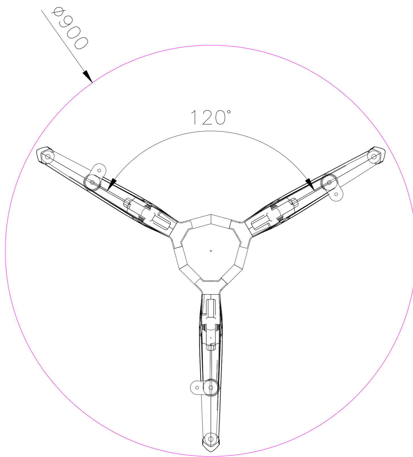
TOP VIEW
