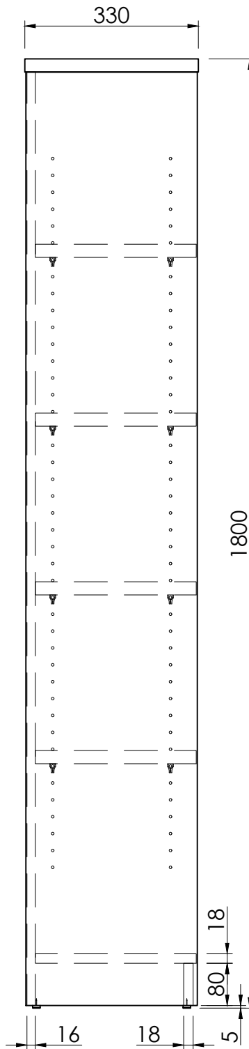
SIDE VIEW
