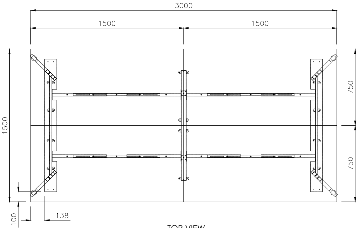
TOP VIEW
