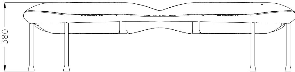
FRONT VIEW
